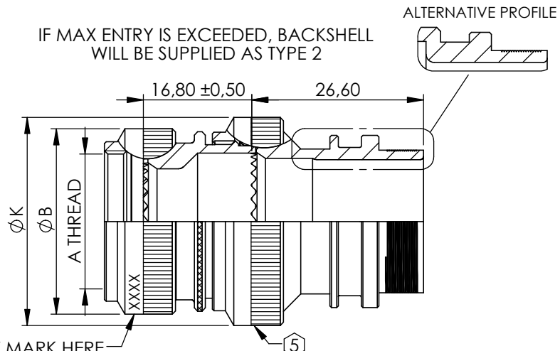
STRAIGHT BACKSHELL - TYPE 2
