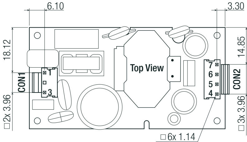
Dimension Drawing “/OF” (mm)
