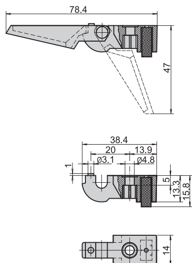
Dimension Drawing
