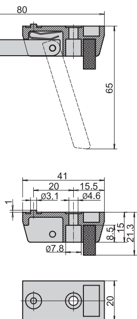
Dimension Drawing
