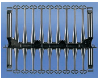
Top view, cable manager with cable fingers front and rear
