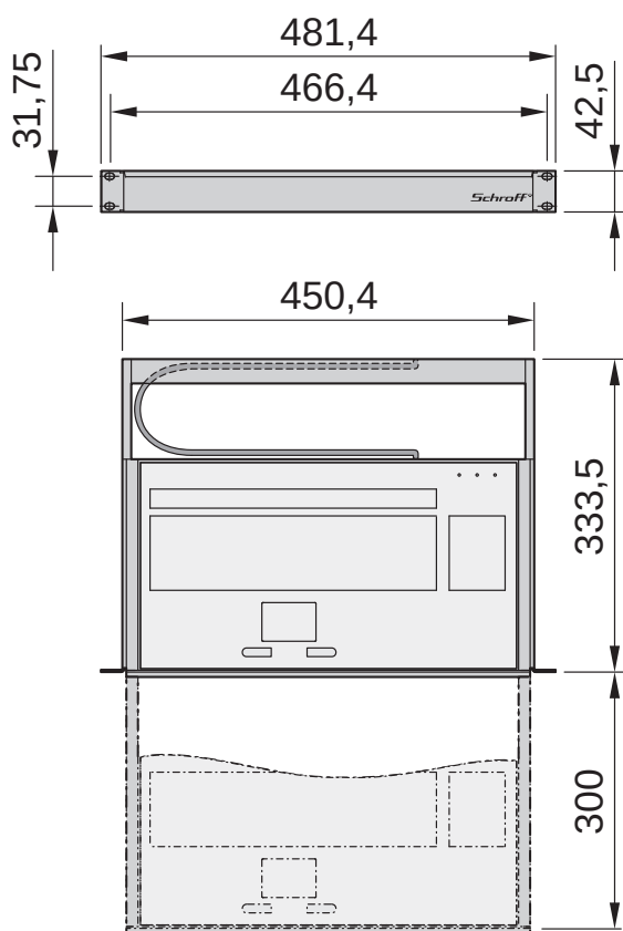
Drawer: Front view, keyboard closed/pulled out
