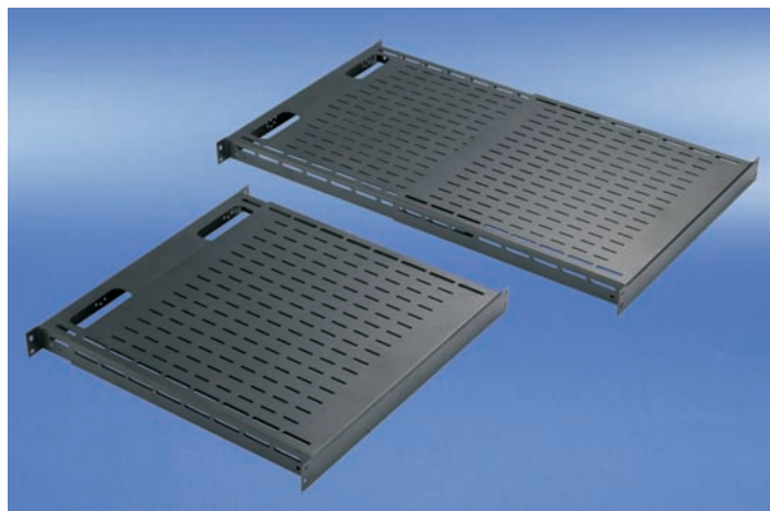
Shelf with variable mounting dimensions
