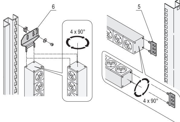
Item 6: bracket for vertical mounting
