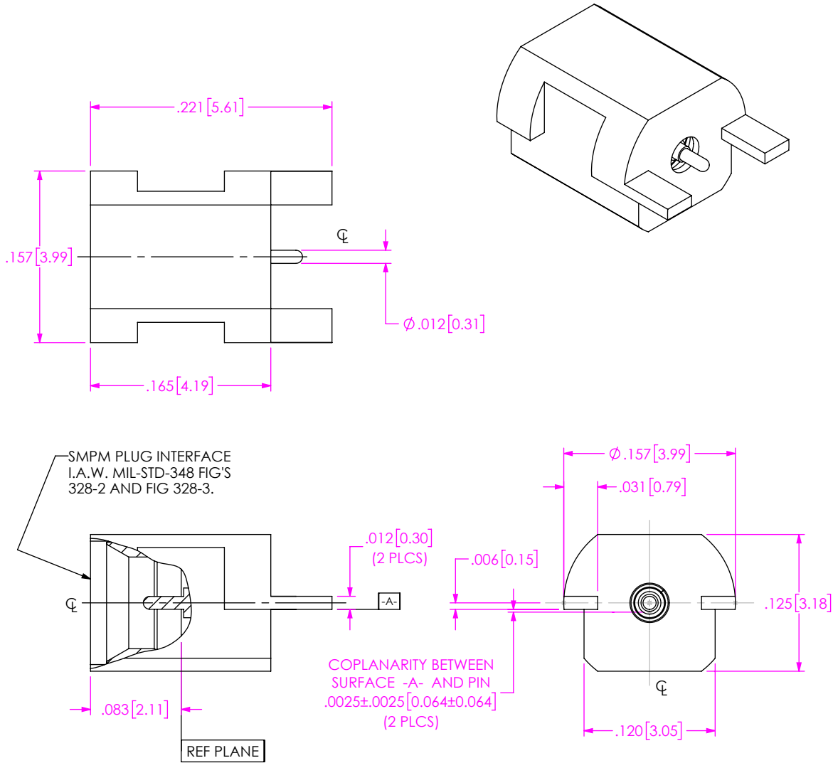
FIG 1 SMPM-PF-P-XX-ST-EM-1 SHOWN
