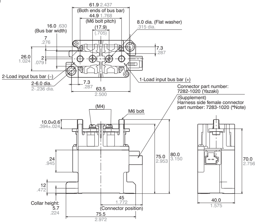
Mounting dimensions
