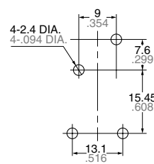
PC board Pattern Tolerance: \pm 0.1 \pm .004
