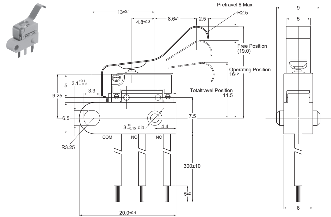
External dimensions
