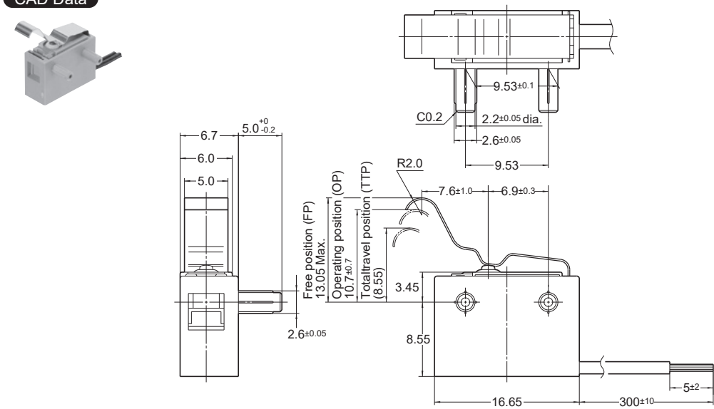
External dimensions
