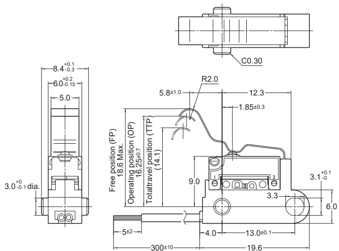
External dimensions
