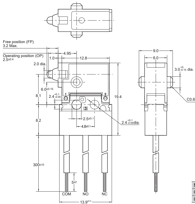
External dimensions
