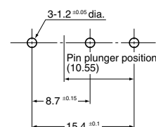
PC board pattern
