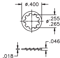
ANTI-ROTATE RING A107 Nickel plated brass 1/4
