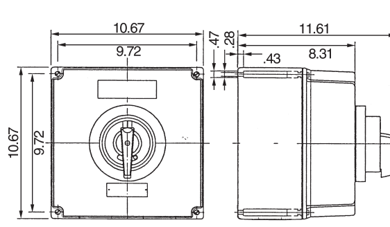
Figure 7 - 80 Amp, 6 Pole
