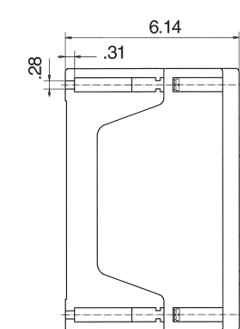
Figure 4 - 40 Amp, 3 Pole
