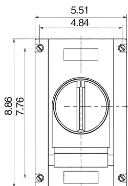
Figure 4 - 40 Amp, 3 Pole
