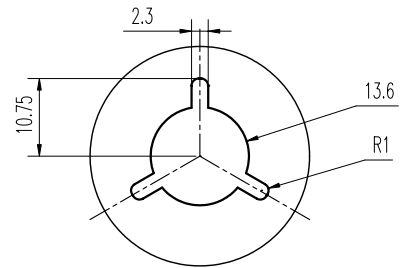
P DETAIL 6:1
