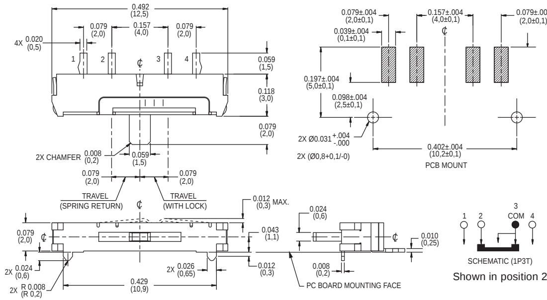
JSM07011SAQN SP3T Surface Mount Momentary one side & Maintained the other
