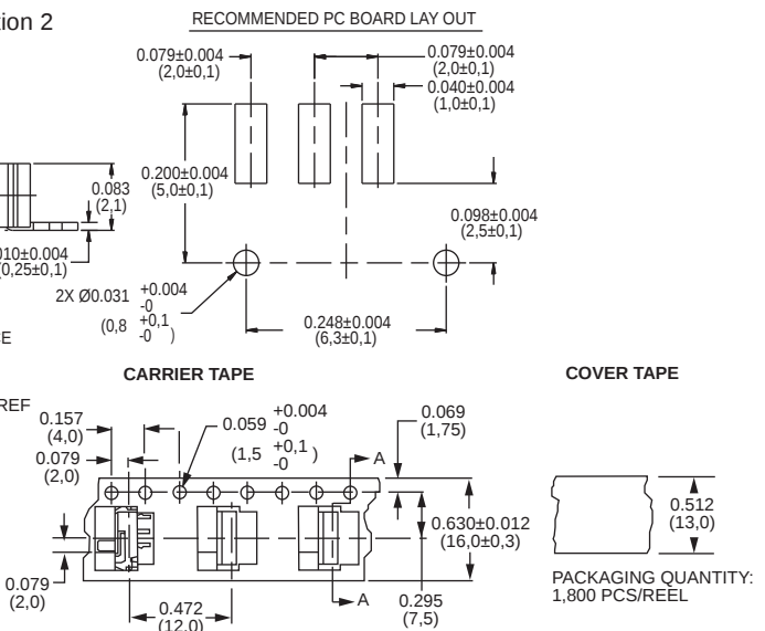
JSM08011SAQNR SPDT Surface Mount Momentary only
