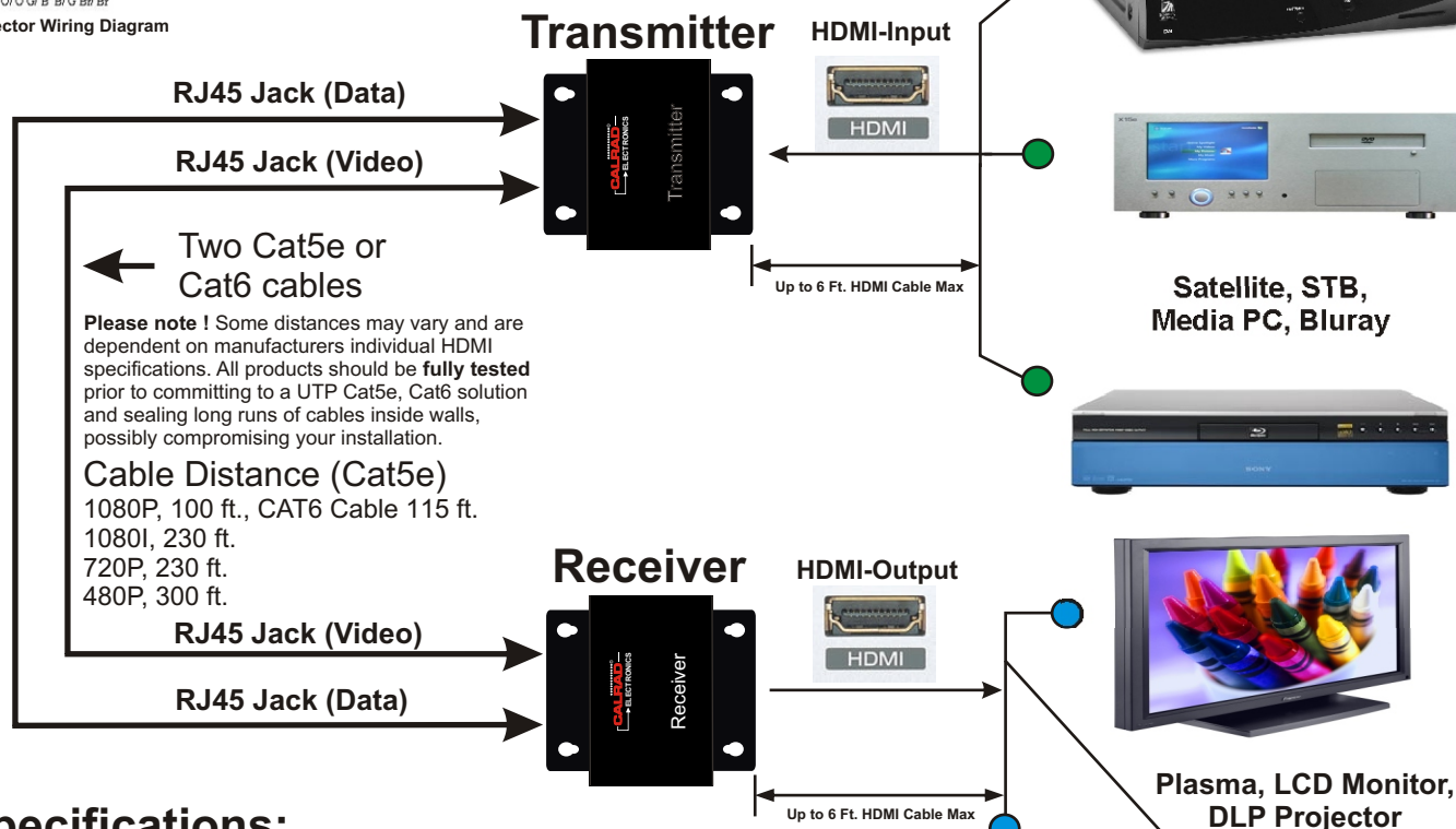
Connector Wiring Diagram
