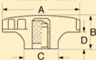
Threaded Insert
