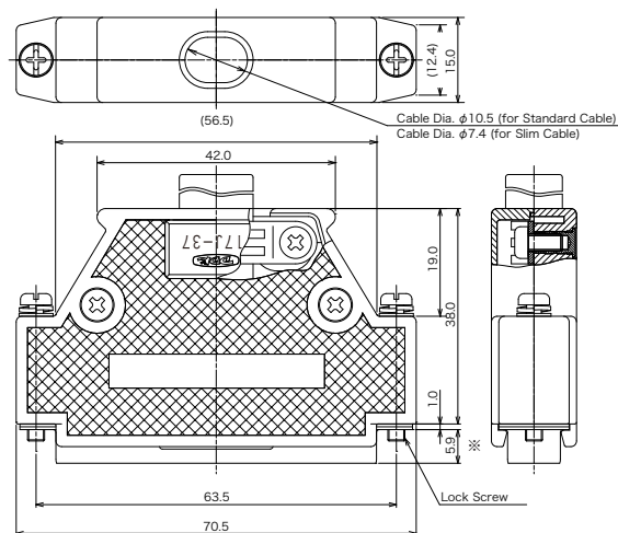
37 contact
