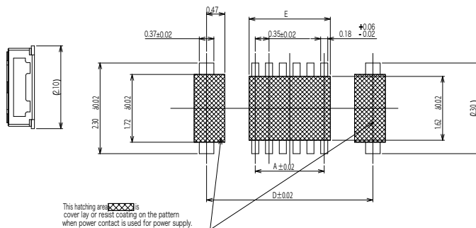
Reference PCB Layout (Connector Mounting Side View)
