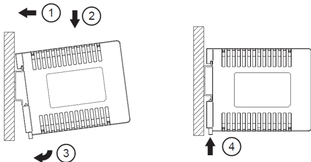
Fig. 2.1 Mounting
