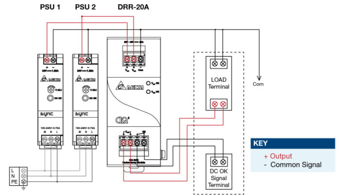
Fig. 3 Redundancy Operation Connection Diagram
