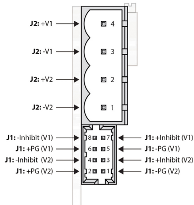
CmG &amp; CmH Output Connectors
