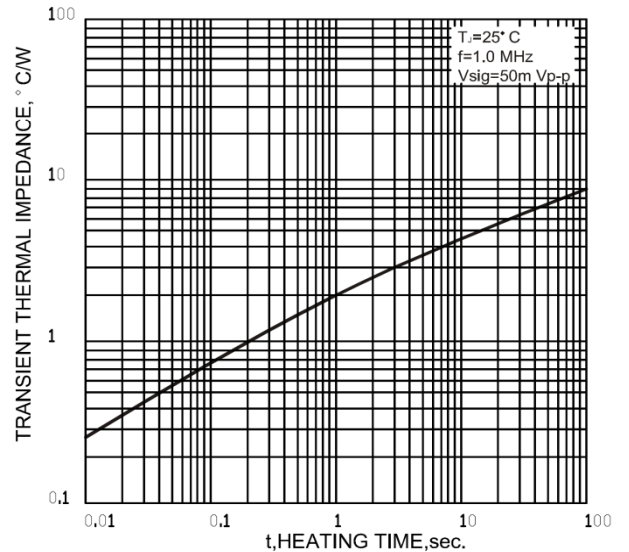
FIG.8-TYPICAL TRANSIENT THERMAL IMPEDANCE PER LEG
