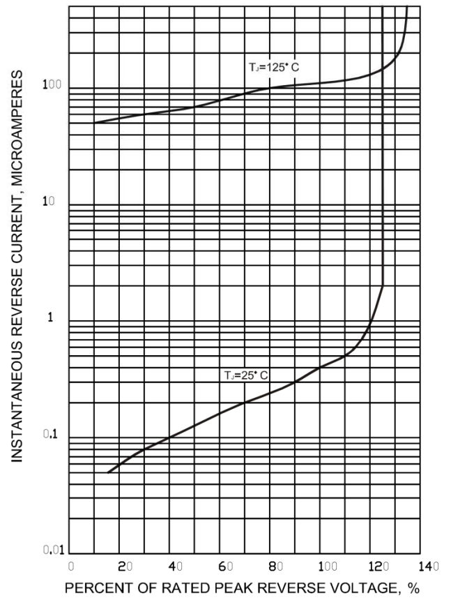
FIG.6-TYPICAL REVERSE CHARACTERISTICS
