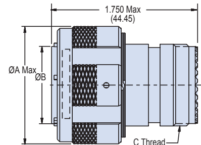
Plug with Male RJ45 Module
