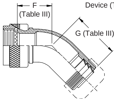
Anti-Rotation Device (Typ.)
