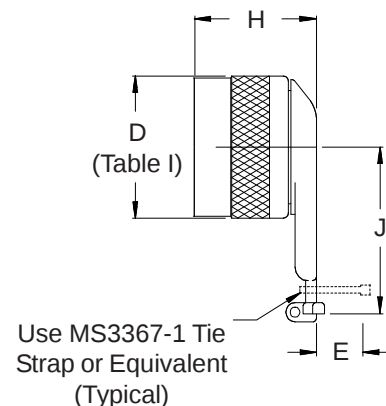
90° ROTATABLE COUPLING
