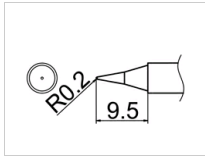
T12-I Shape-I
