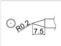
T12-B Shape-B
