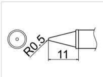
T12-WB2 Shape-0.5WB * Heavy Duty Type
