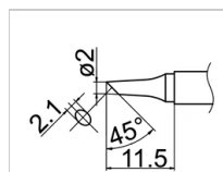
T12-BC2 Shape-2BC
