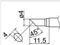
T12-CF4 Shape-4C Tinned cut surface only
