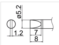
T12-D52 Shape-5.2D
