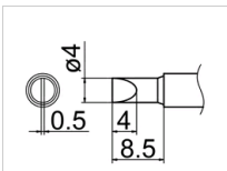
T12-D4 Shape-4D
