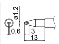
T12-DL12 Shape-1.2DL
