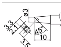
T12-BCM3 Shape-3BC Bevel with indent
