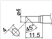
T12-C4 Shape-4C
