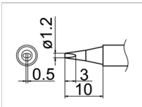
T12-D12 Shape-1.2D
