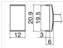
T12-1010 Tunnel Size 19.5 x 12
