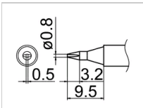
T12-D08 Shape-0.8D
