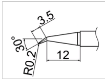
T12-J02 Shape-0.2J
