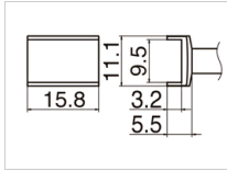
T12-1004 Tunnel Size 9.5 x 15.8
