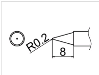
T12-BZ Shape-B(Z) * Long Life Type
