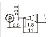
T12-WD08 Shape-0.8WD
