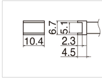
T12-1002 Tunnel Size 5.1 x 10.4
