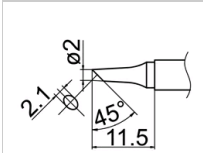
T12-BCF2 Shape-2BC Tinned cut surface only
