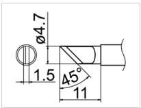
T12-KL Shape-KL For drag soldering for left-handed.
