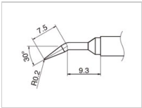
T12-JL02 Shape-0.2JL
