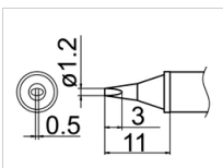
T12-WD12 Shape-1.2WD
