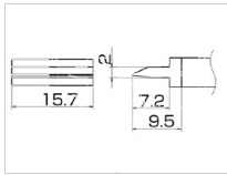
T12-1402 Spatula Size 15.7
