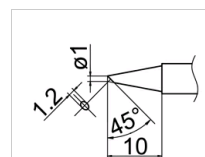
T12-BCF1Z Shape-1BC(Z) * Long Life Type
