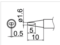
T12-D16Z Shape-1.6D(Z) * Long Life Type
