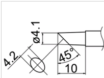
T12-C4Z Shape-4C(Z) * Long Life Type
