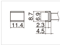
T12-1006 Tunnel Size 6.9 x 11.4
