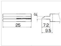
T12-1404 Spatula Size 25
