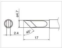
T12-KF Shape-KF
