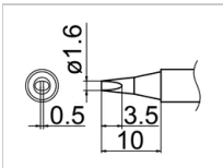
T12-D16 Shape-1.6D
