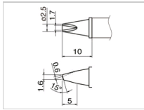
T12-1610 Concave
