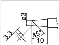
T12-BCF3 Shape-3BC Tinned cut surface only
