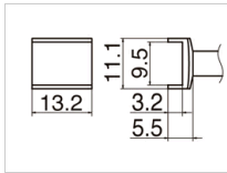
T12-1005 Tunnel Size 5.1 x 13.2
