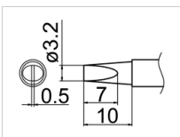
T12-DL32 Shape-3.2DL
