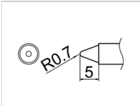
T12-B3 Shape-0.7B
