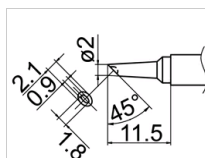
T12-BCM2 Shape-2BC Bevel with indent
