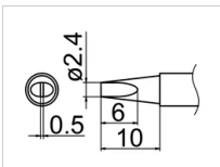
T12-D24Z Shape-2.4D(Z) * Long Life Type
