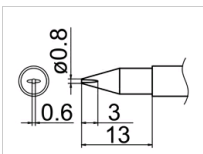
T12-DL08 Shape-0.8DL
