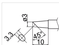
T12-BC3 Shape-3BC
