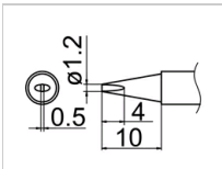
T12-D12Z Shape-1.2D(Z) * Long Life Type
