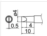
T12-D4Z Shape-4D(Z) * Long Life Type
