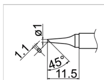
T12-BC1 Shape-1BC
