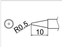
T12-B2 Shape-0.5B
