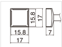
T12-1208 Quad Size 15.8 x 15.8
