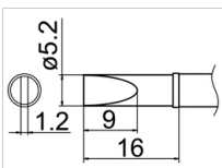
T12-DL52 Shape-5.2DL
