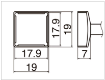
T12-1204 Quad Size 17.9 x 17.9
