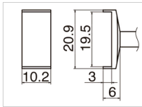
T12-1008 Tunnel Size 19.5 x 10.2
