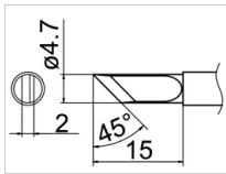
T12-K Shape-K
