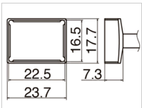
T12-1206 Quad Size 22.5 x 16.5
