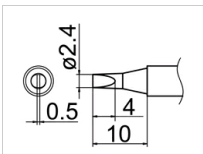
T12-D24 Shape-2.4D
