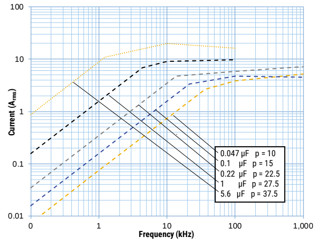
1,000 VDC/600 VAC
