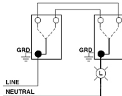
Wiring Diagram 3-Way to 3-Way
