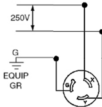
Wiring Diagram
