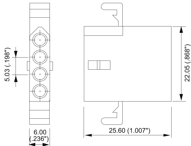
Receptacle ( 37-404-0 )
