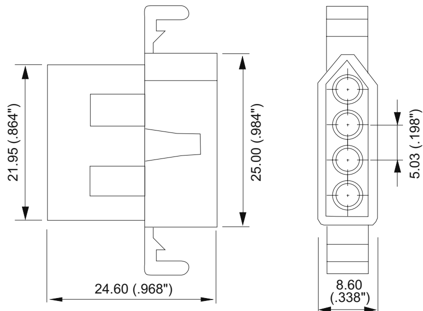
Plug ( 37-304-0 )
