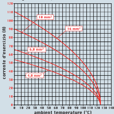
diagram CX 4/2 poles
