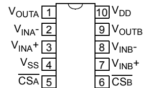
MCP665 MSOP
