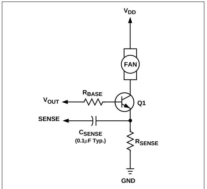
Figure 7. SENSE Network
