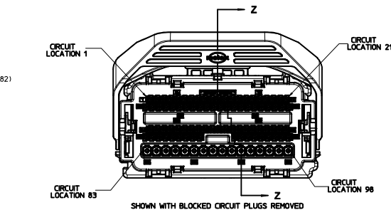
SHOWN WITH BLOCKED CIRCUIT PLUGS REMOVED
