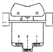
TP Series Rocker Switch, 4 pole, 3 position, Screw terminal, Flush Panel Mounting
