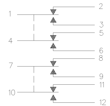
CIRCUIT DIAGRAM
