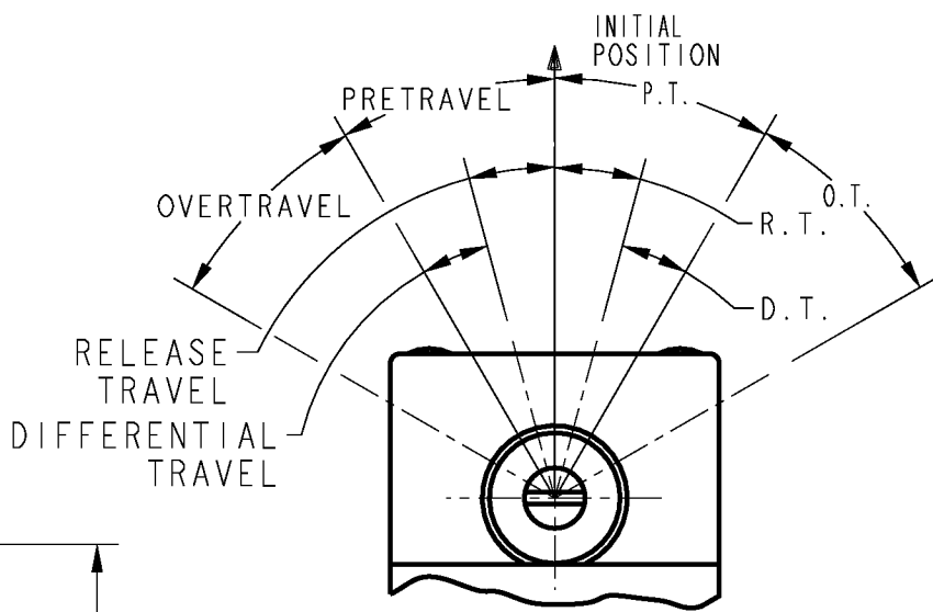
OPERATING DATA - SIDE ROTARY
