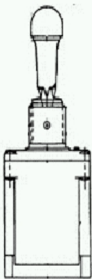
TL Series Toggle Switch, 2 pole, 2 position, MTS (14-16 Gage) terminal, Locking Lever, Military Part Number MS27782-23G
