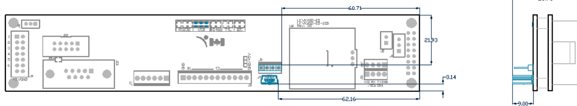
Figure 23: USB Model Dimensional Drawing
