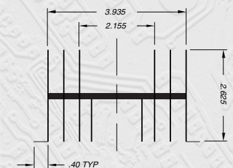
Accessory Heat Sink Part No. ASY-HS25A-011
