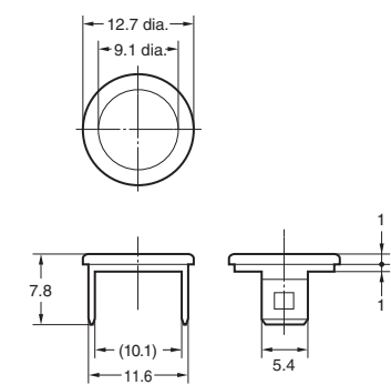
Flange (Round) A3A-25
