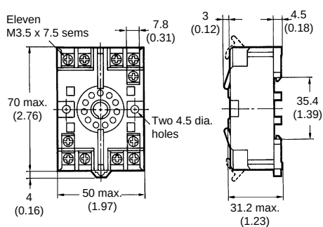
Terminal Arrangement
