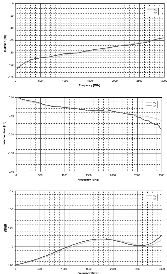
RF performance, 50Ω version
