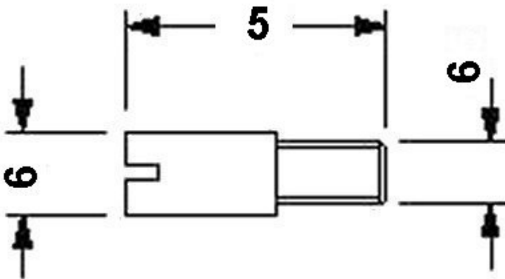
Dimensional drawing
