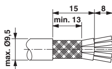
Dimensional drawing
