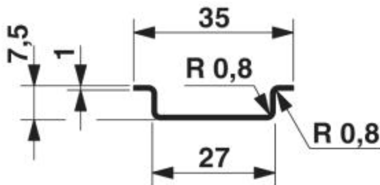
Dimensional drawing
