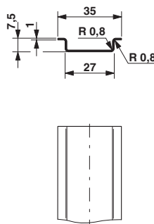
Dimensional drawing
