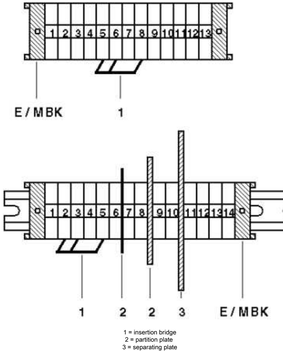
Circuit diagram
