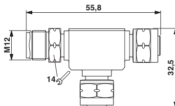
Dimensional drawing
