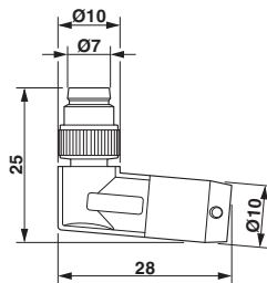
M8 x 1 male plug, angled version
