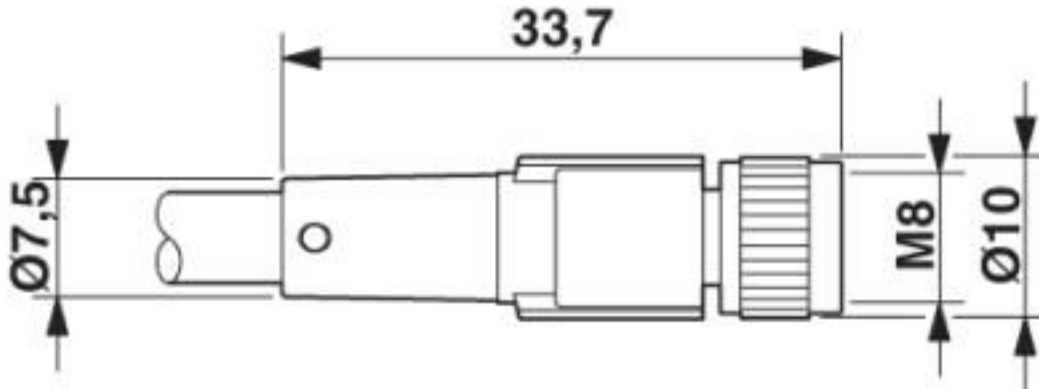
Dimensional drawing
